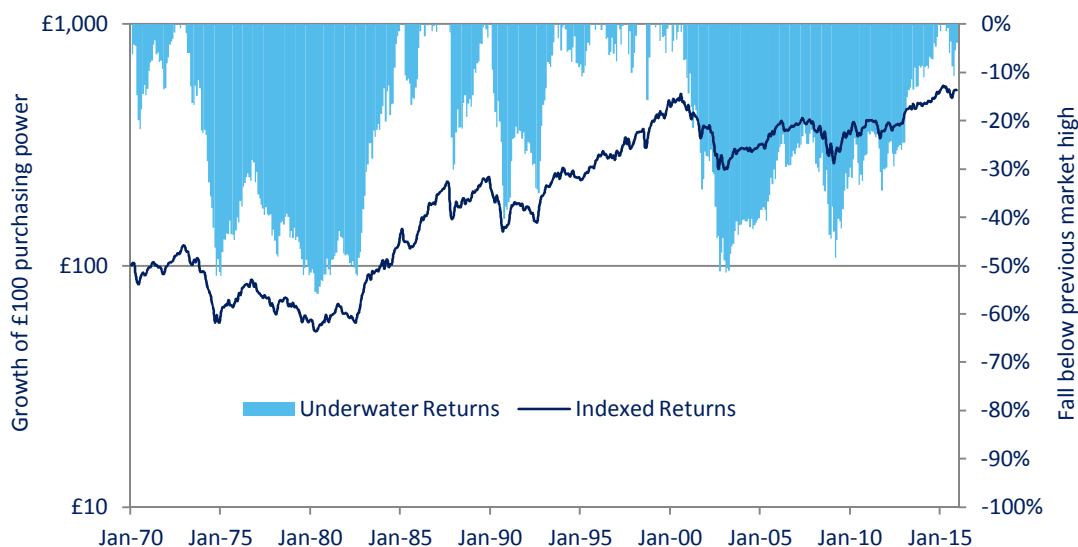
Figure 2: The depth and longevity of being below a previous market high (1970 – 2015)
